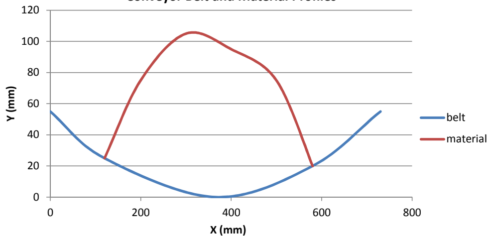
Conveyor Belt and Material Profiles
